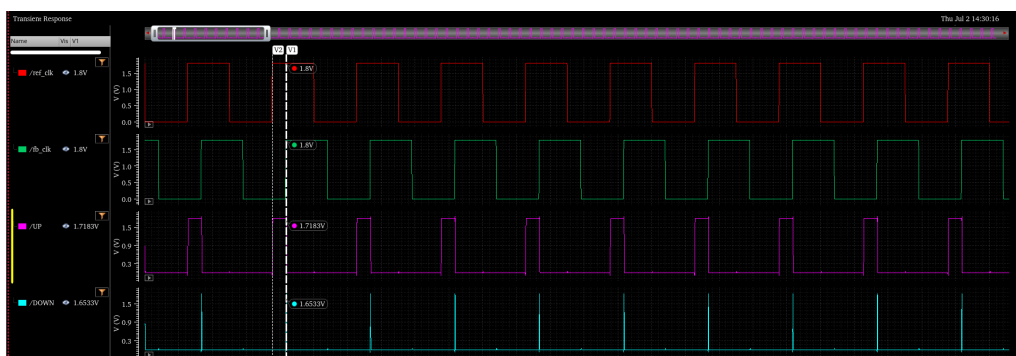
Figure 4.1: Simulation result of the Phase Frequency Detector.
