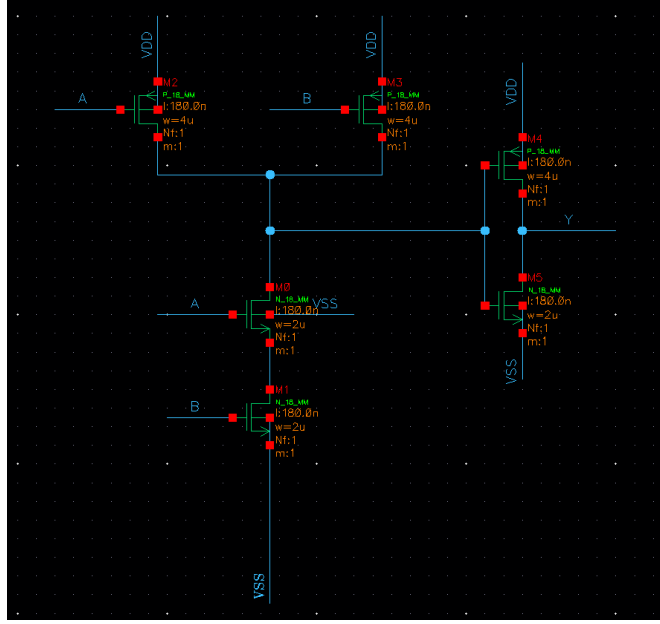
Figure 3.4: Transistor-level schematic of the CMOS AND gate.
