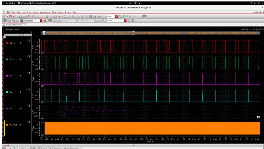
Figure 4.5: Simulation result of the complete Phase Locked Loop.
